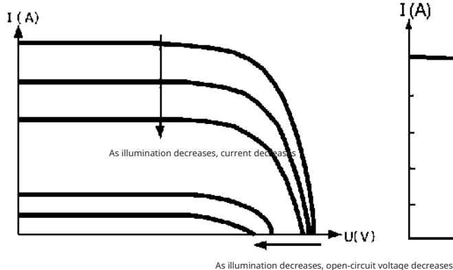
Figure 1-3 Relationship between solar panel output characteristics and light intensity
