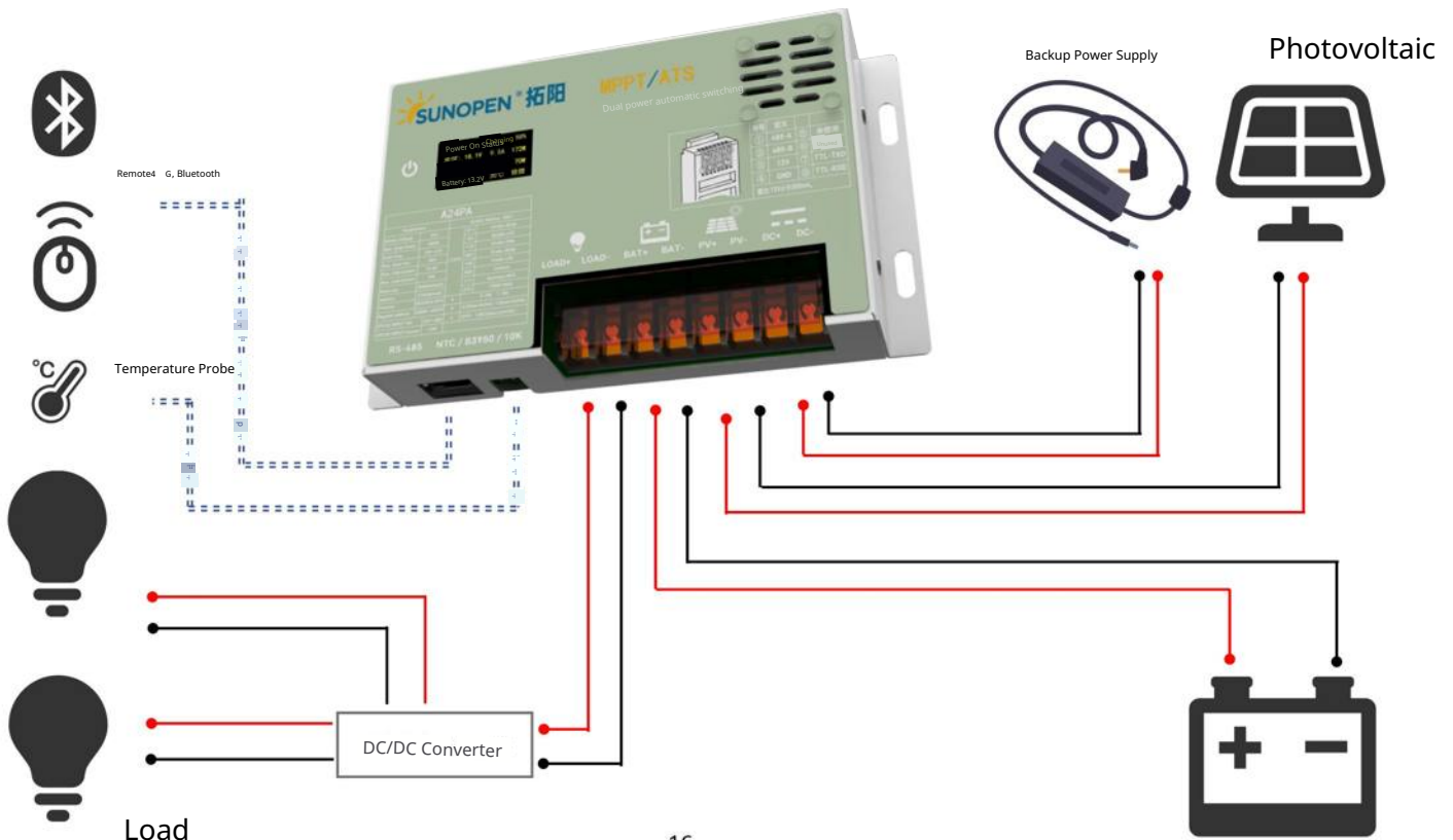
A24PB (MPPT+ATS)
