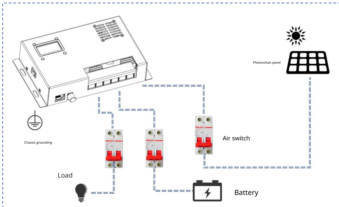
13. Application wiring diagram
